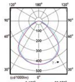
SM136V NOC
