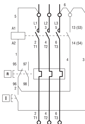
Diagram 1 - Incorporated button control
