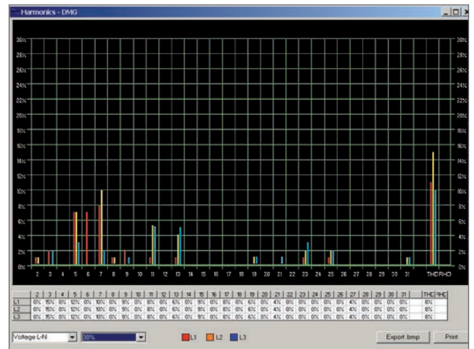
Harmonic analysis in bar-graph and table format
