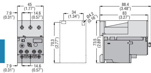
RF...200 thermal relay with links
