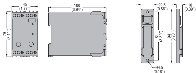
DRPT relay
