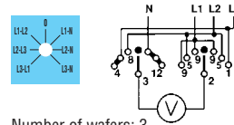
66 - Phase-phase phase-neutral voltmeter changeover / double throw
