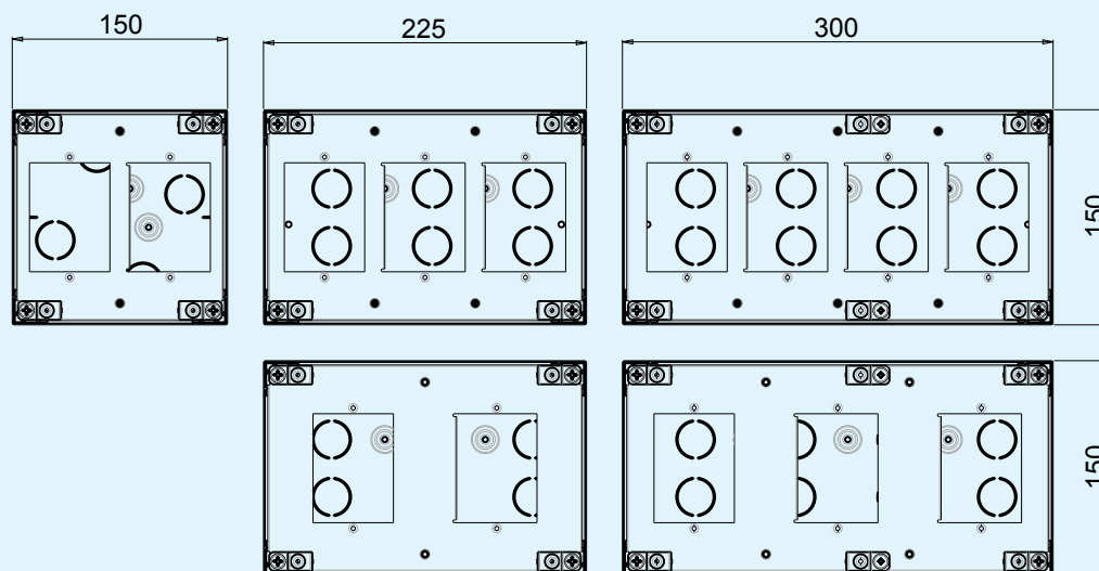
Standard Wall Box Dimensions
