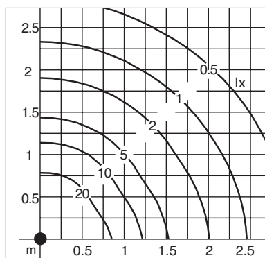
ATTORNO SYMMETRICAL 26W CFL H=0.72M
