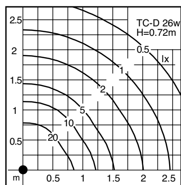
ATTORNO SYMMETRICAL 18W CFL H=0.72M
