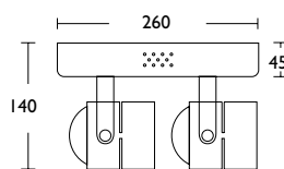
Head dimensions: 80(l)mm x 58(w)mm
