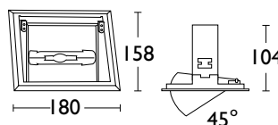
Cut-out: 140mm x 160mm
