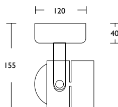
Head dimensions: 80(l)mm x 58(w)mm
