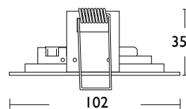
Cut-out: 95mm
