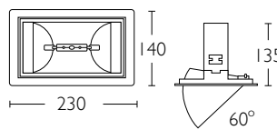
Cut-out: 215mm x 125mm
