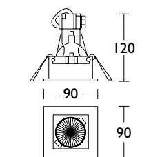
Cut-out: 82mm x 70mm
