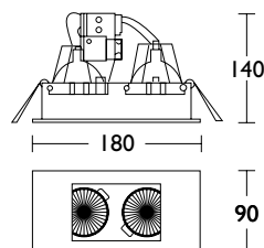
Cut-out: 172mm x 70mm
