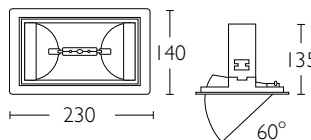
Cut-out: 215mm x 125mm
