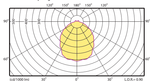
Polar intensity diagram
