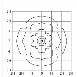
City Light Plus LED Symmetric H = 4.5m
