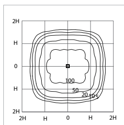
Cardinal LEP Highbay H = 6m
