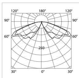
City Light Bollard LED —C0 - C180 - - -C90 - C270
