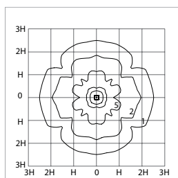
City Light Elegance LED Symmetric H = 4.5m
