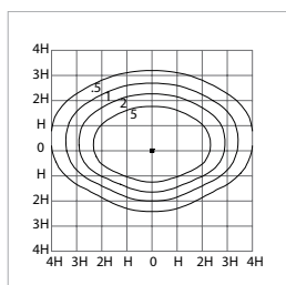
A2 Midi LED 103W H = 4.5m
