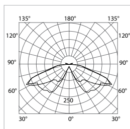
City Light Elegance LED — C0 - C180 --- C90 - C270
