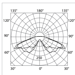
Lantern LED —C0 - C180 ---C90 - C270
