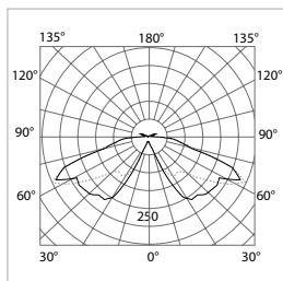
City Light Plus LED — C0 - C180 --- C90 - C270
