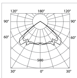
Cardinal LEP Highbay —C0 - C180 ---C90 - C270
