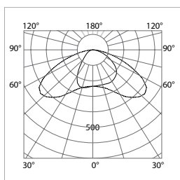
A2 Midi LED 103W — C0 - C180 - - - C90 - C270
