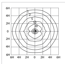
City Light Bollard LED H = 1.5m
