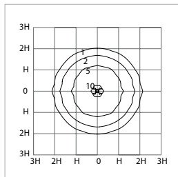
DL20 3K LED Symmetric H = 4.5m
