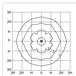
Lantern LED Symmetric H = 4.5m
