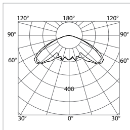
DL20 3K cd/klm — C0 - C180 -- C90 - C270
