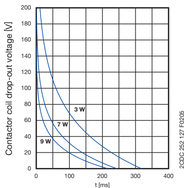
Time delay guideline values 200-240 V AC version without jumper 3/4
