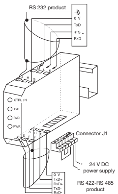
RS 422 - RS 485 4 WIRE SERIAL LINKS
