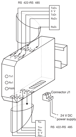
RS 422 - RS 485 4 wire serial link
