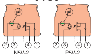
1 A output optocoupler 5 V DC
