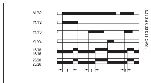
Function diagram CM-KRN
