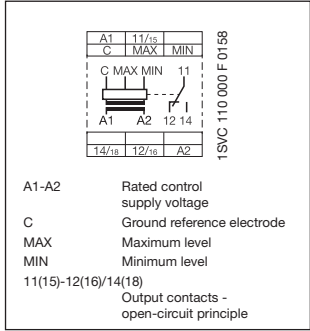
Connection diagram CM-ENS
