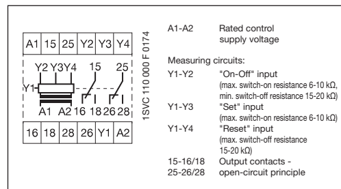
Connection diagram CM-KRN
