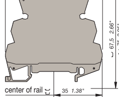
Spring clamp module
