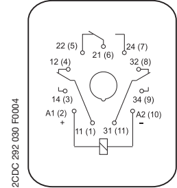
CR-U with 3 c/o contacts
