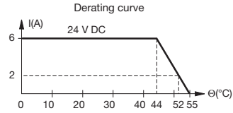
Limited load in CC
