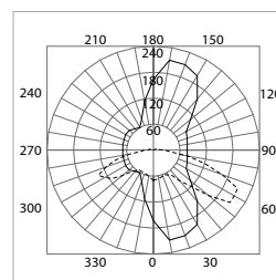
B2001 Nostalgia 70HPS .... Vertical Plane Through Horizontal Angles (10-190) — Horizontal Cone Through Vertical Angle (62.5) cd/km
