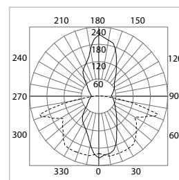
Bourke Hill Eco - A 42W CFL ... Vertical Plane Through Horizontal Angles (270-90) — Horizontal Cone Through Vertical Angle (72.5) cd/klm
