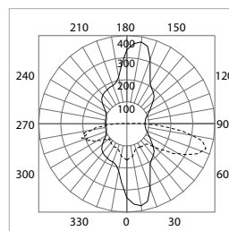
Nostalgia 70MH --- Vertical Plane Through Horizontal Angles (10-190) --- Horizontal Cone Through Vertical Angle (62.5) cd/klm
