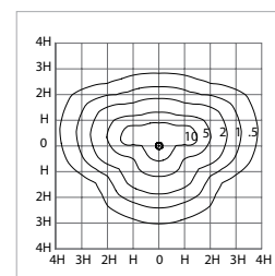
B2001 Nostalgia Series 70HPS H = 4.5m
