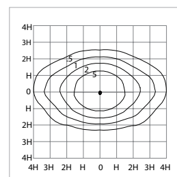
Bourke Hill Eco - A 42W CFL H = 4.5m
