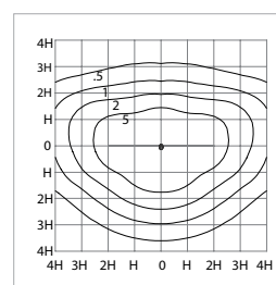
Bourke Hill - S 100W MH H = 4.5m
