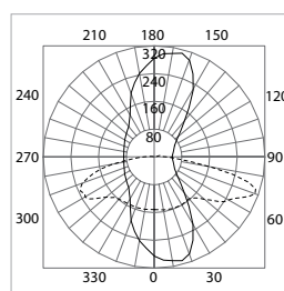
Bourke Hill - S 100W MH --- Vertical Plane Through Horizontal Angles (255-75) — Horizontal Cone Through Vertical Angle (70) cd/klm
