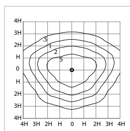
Kensington 70HPS H = 4.5m
