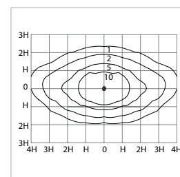
Parkville - S 250 HPS H = 12m Upcast 0
