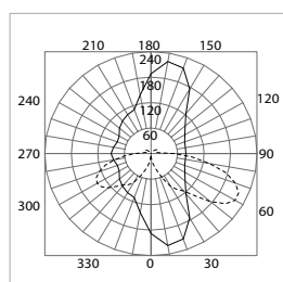
Kensington 70HPS ..... Vertical Plane Through Horizontal Angles (10-190) ——— Horizontal Cone Through Vertical Angle (62.5) cd/klm
