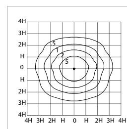
Avenue 42W H = 4.5m
