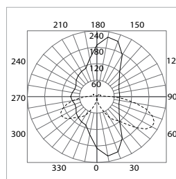
Kensington Longreach 70HPS --- Vertical Plane Through Horizontal Angles (10-190) --- Horizontal Cone Through Vertical Angle (62.5) cd/klm
