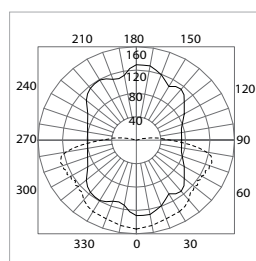
Avenue 42W CFL --- Vertical Plane Through Horizontal Angles (10-190) --- Horizontal Cone Through Vertical Angle (62.5) cd/klm
