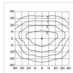
Nostalgia 70W MH H = 4.5m
