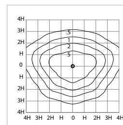
Kensington Longreach 70HPS H = 4.5m
