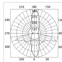
Parkville-S 250HPS --- Vertical Plane Through Horizontal Angles (10-190) --- Horizontal Cone Through Vertical Angle (62.5) cd/km
