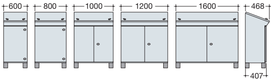
DESK SWITCHBOARD
