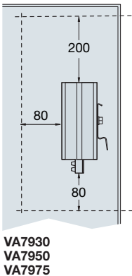
Minimum mounting distances
