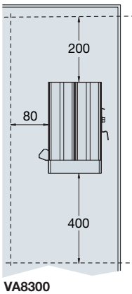
Minimum mounting distances
