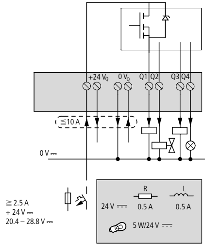
Figure 30: Transistor outputs CL-LST
