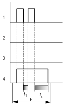
Figure 65: Signal diagram of timing relay, off-delayed (with/without random switching with retriggering)
