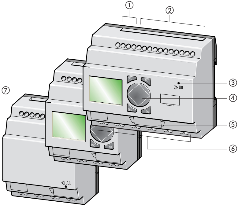
Figure 2: Device overview
