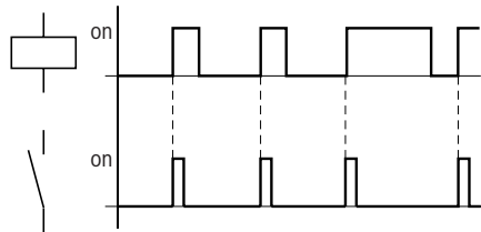
Figure 42: Signal diagram of cycle pulse with rising edge
