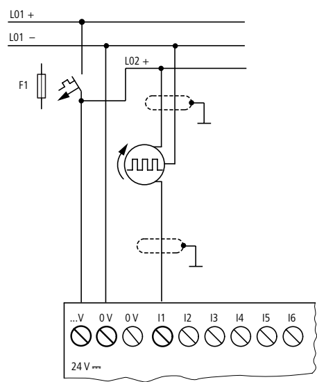
Figure 25: Connecting high-speed counters and frequency generators
