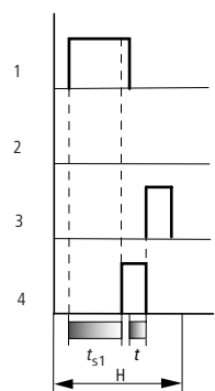
Figure 68: Signal diagram timing relay, on- and off-delayed 3
