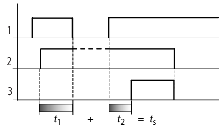
Figure 72: Function of the circuit
