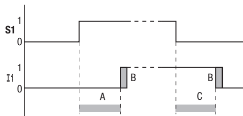
Figure 82: Delay times of CL-DC1 and CL-DC2 basic units
