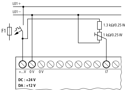
Figure 21: Analog setpoint potentiometer with 24 V DC power feed
