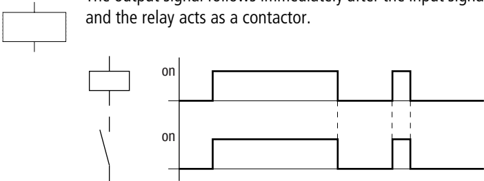
Figure 39: Signal diagram of contactor function
