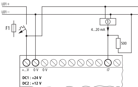
Figure 24: Connection 0 (4) to 20 mA sensor output, analog input
