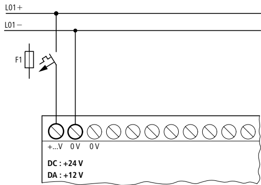
Figure 9: Supply voltage to DC basic unit
