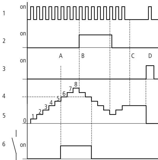
Figure 53: Signal diagram
