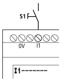
Figure 81: CL input assigned with a switch
