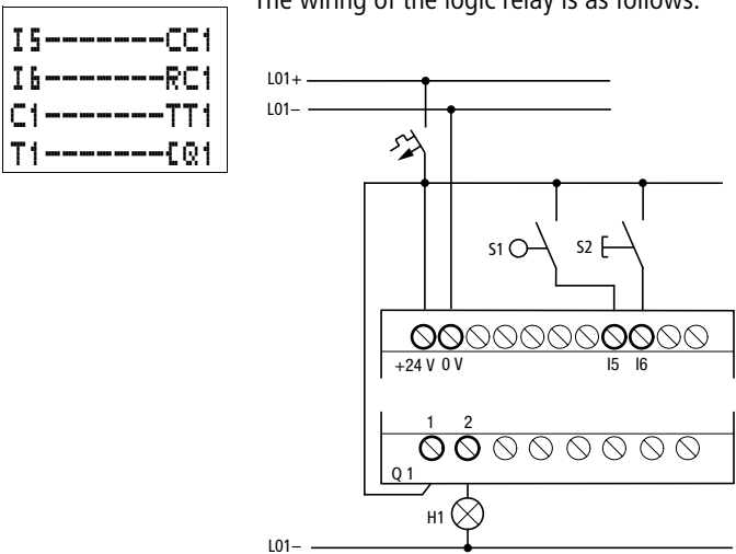
Figure 46: CL wiring and circuit diagram
