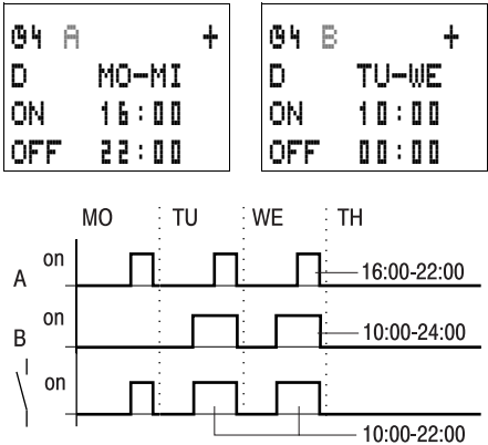
Figure 61: Time overlaps signal diagram
