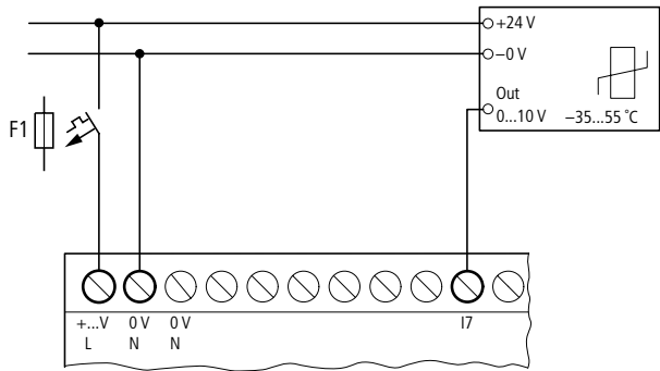
Figure 23: Connection of the temperature sensor, analog input
