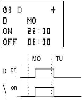
Figure 60: Night switching signal diagram
