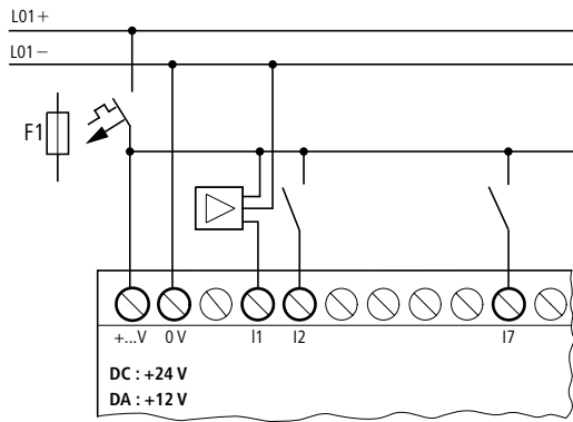
Figure 17: Connect digital inputs CL-DC1 and CL-DC2
