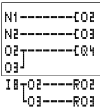
Circuit diagram display
