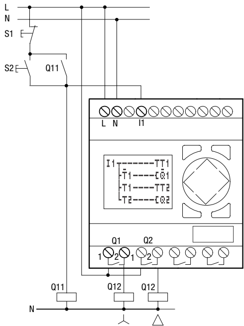
Figure 74: Star-delta circuit with the logic relay
