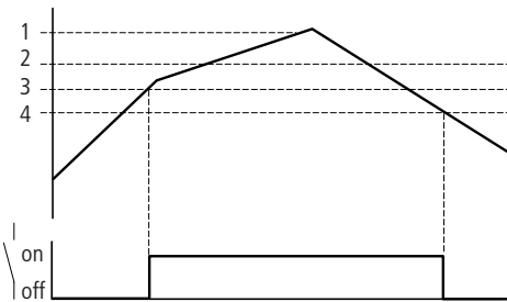
Figure 51: Signal diagram of analog value comparator in Greater than/equal to mode
