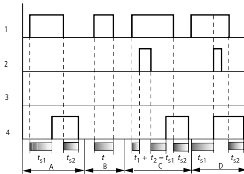
Figure 66: Signal diagram timing relay, on and off-delayed 1
