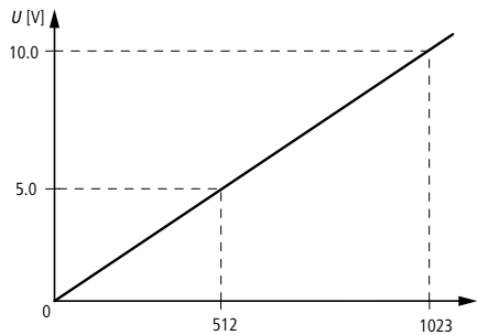
Figure 47: Resolution of the analog inputs
