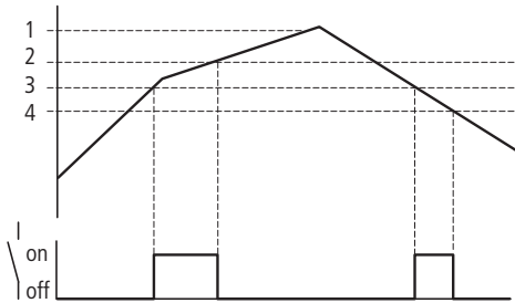
Figure 50: Signal diagram of analog value comparator in Equal to mode
