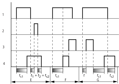
Figure 67: Signal diagram timing relay, on and off-delayed 2
