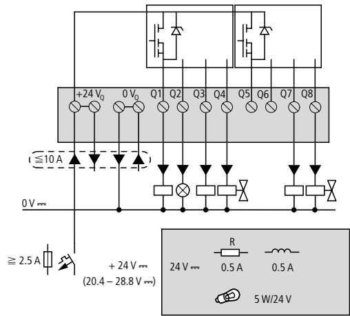
Figure 31: Transistor outputs CL-LMT
