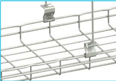
3 AS - Hangers
