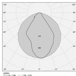
53W 4000K ASYMMETRICAL
