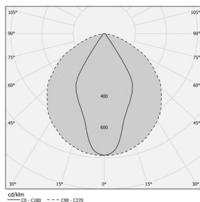
53W 4000K SYMMETRICAL
