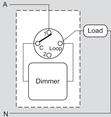
One-way switching with dimmer
