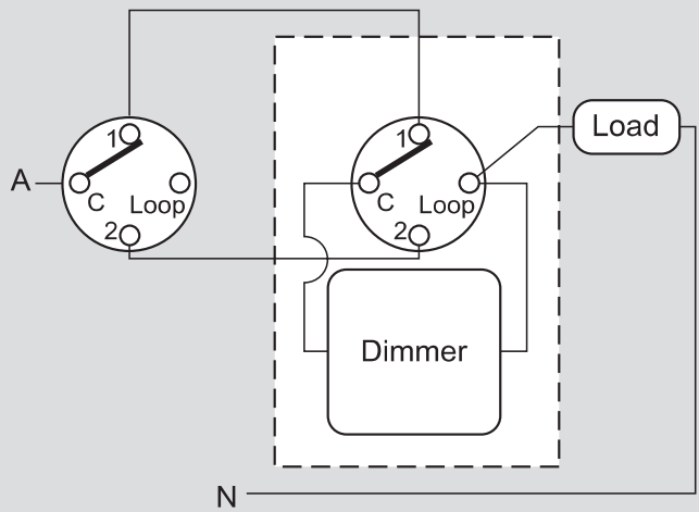
Two-way switching with dimmer
