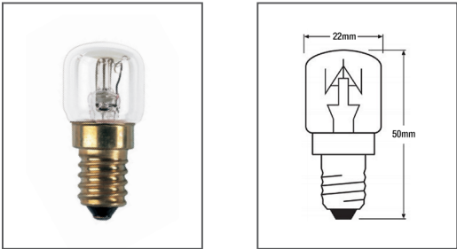
SPC.T OVEN CL 15 W E14 SPECIAL OVEN T | Incandescent lamp, tubular shape, for oven and pilot lighting. Available in 15W clear with E14 base.
