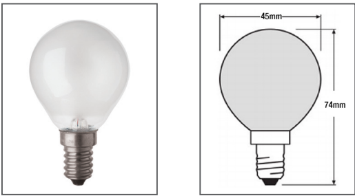
SPC.P OVEN FR 40 W E14 SPECIAL OVEN P | Incandescent lamps, classic mini-ball shape, for oven lighting. Available in 40W frosted with E14 base.
