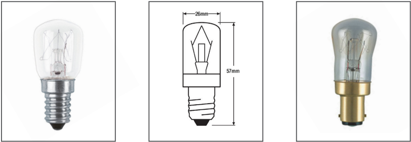
SPECIAL T/FRIDGE Incandescent lamp, tubular shape pilot light for fridges, sewing machines and range hoods. Available in 15W/25W clear and 15W frosted in E14/B15d bases.
