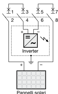
Wiring diagram of a PV plant downstream the strings S 284 UC - IT system
