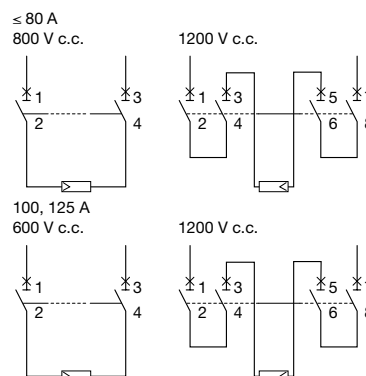
Use of S800 PV-S thermal magnetic CBs in DC Layout of PV panels in earth-insulated systems
