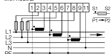
DAB12000 Three-phase system without neutral
