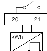
Impulsive output active energy metering
