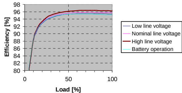
Galaxy 3500 30kVA Efficiency
