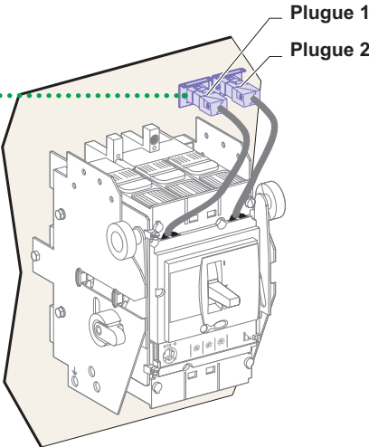
Compact NSX100/160/250.
