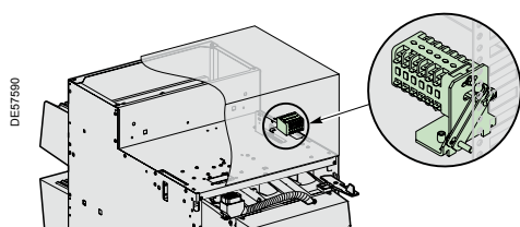
Indication contacts
