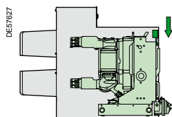
Disconnected position
