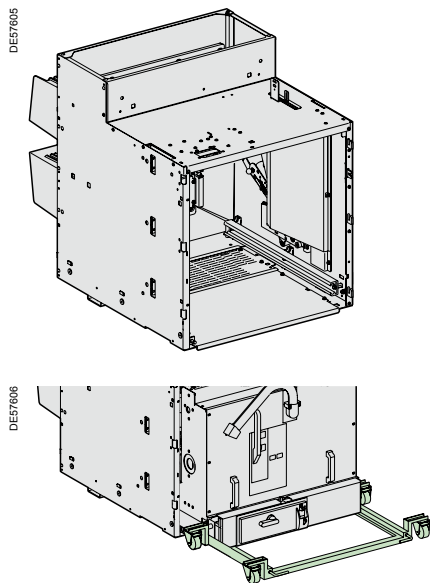
Extraction tool
