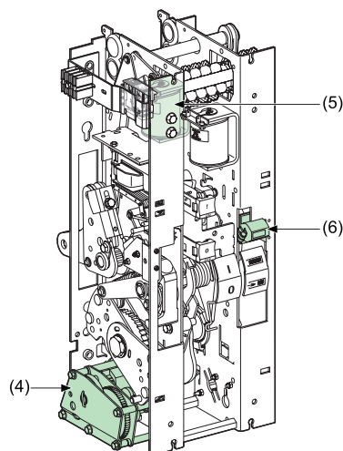
Operating mechanism
