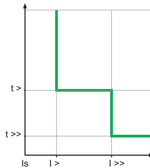
With a definite time lower threshold
