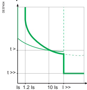
With an inverse definite time lower threshold
