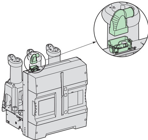
LV connection with plug
