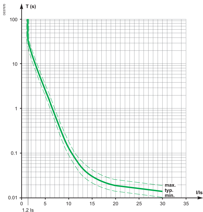
Phase protection trip curve: VIP30 and VIP35
