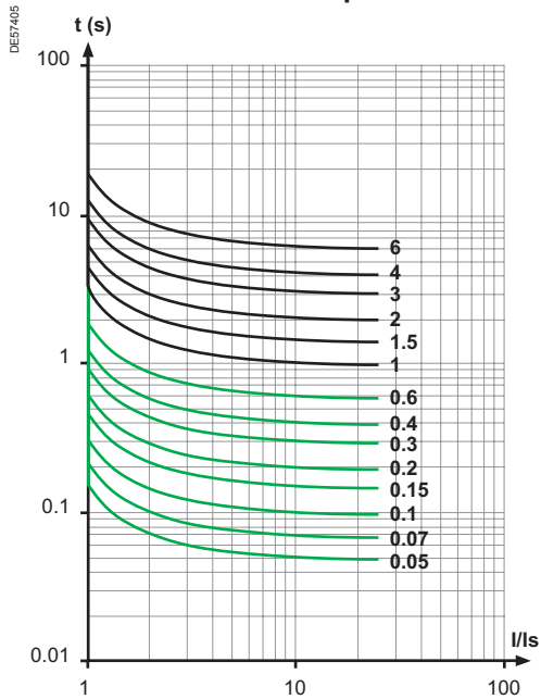
RI curve
