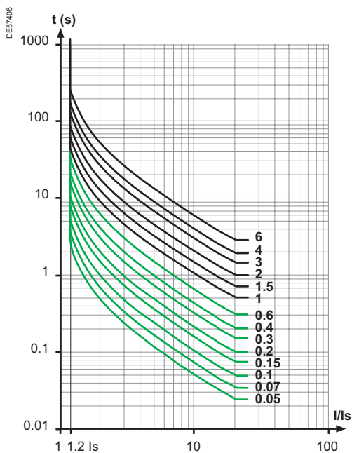
VI curve
