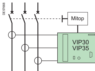
Simplified connection arrangement
