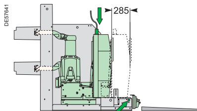
Service position
