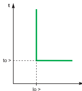
VIP35: earth protection curve
