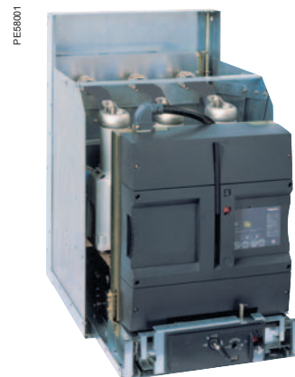
Evolis 24 kV withdrawable, frontal version in NEX cradle
