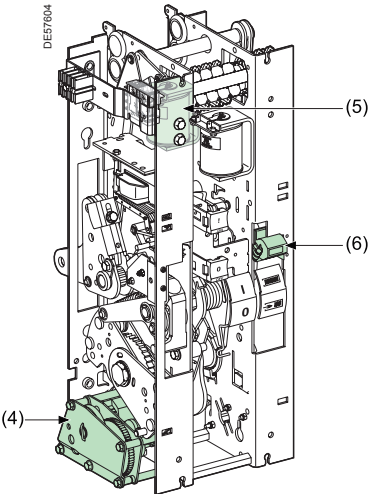
Operating mechanism
