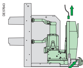
Disconnected position
