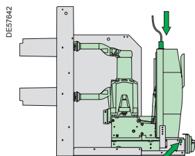
Test position
