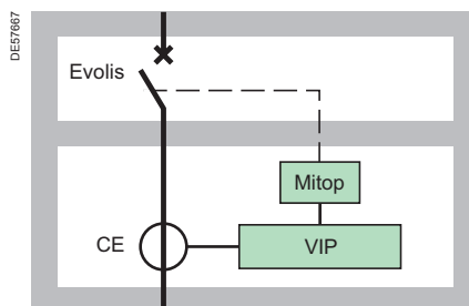
EVOset schematic diagram
