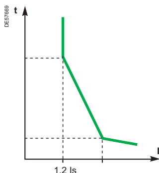
VIP30/VIP35: phase protection curve
