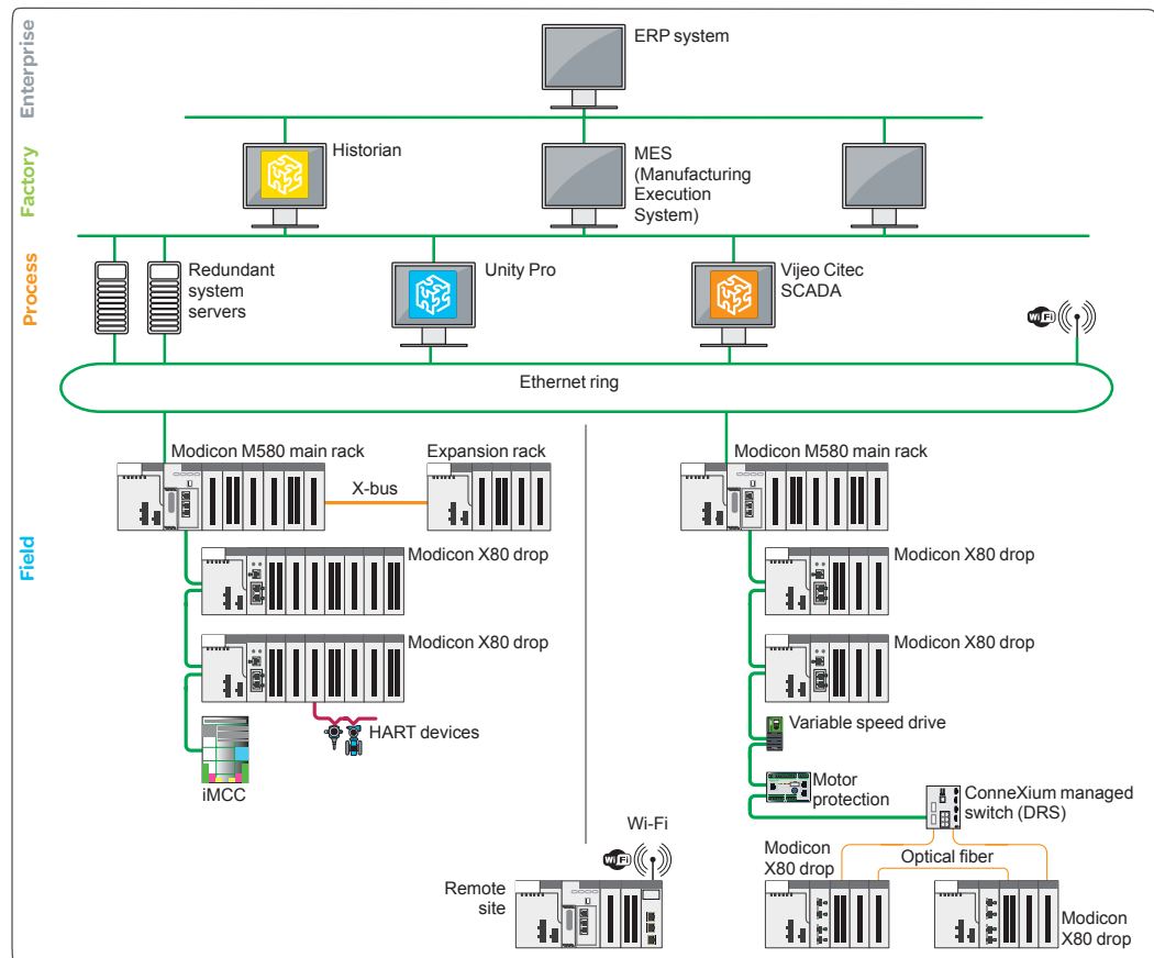
Typical architecture (3)
