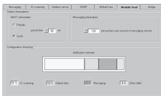
Bandwidth management
