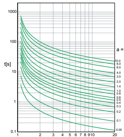
Normal inverse
