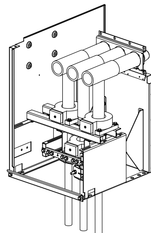
CB cable compartment with metering CT cores
