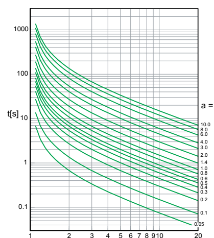
Very Inverse
