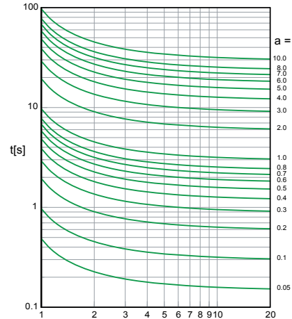
RI Inverse
