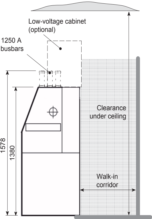
Space under ceiling with top-mounted LV cabinet.
