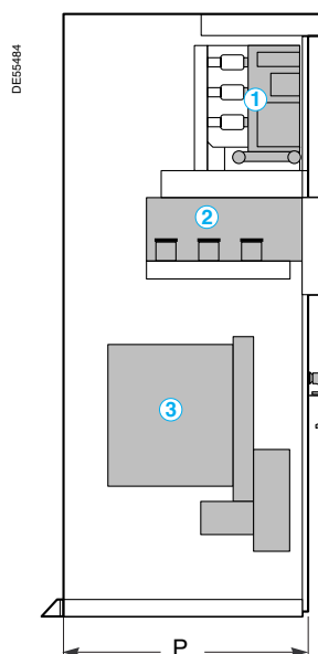
Vista lateral soft starter
