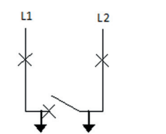
ATS100-BTA: 2 line incomers with bus tie
