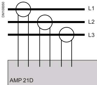
Connection diagram
