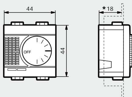
SONDA LIVING/LIGHT
