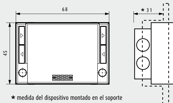
CENTRAL ART. HC/HS4695
