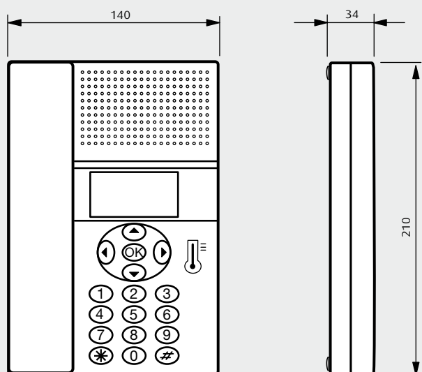
CENTRAL ART. 3550
