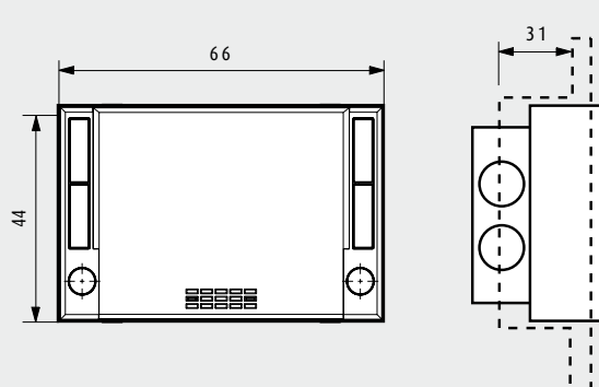
CENTRAL ART. L/N/NT4695
