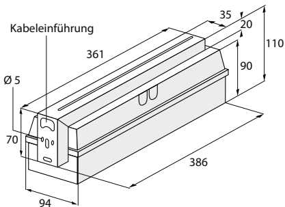
Optima 14L A (SL)
