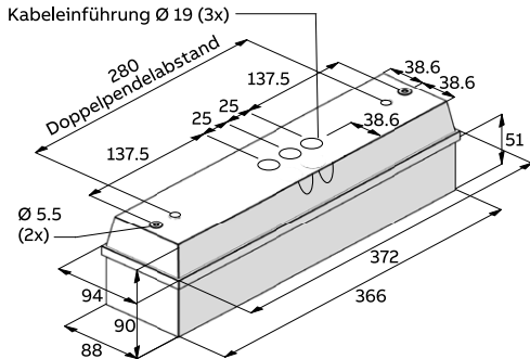
Optima 14L A (SL)
