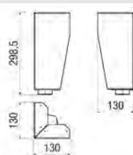
Maße [mm]
