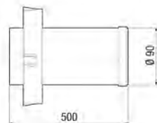
Maße [mm]
