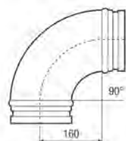
Maße [mm]
