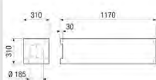
Maße [mm]
