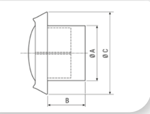
Maße [mm]
