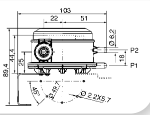
Maße [mm]
