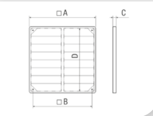
Maße [mm] AS 65 Ex bis AS 71 Ex
