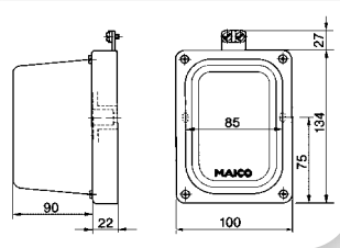
Maße [mm]
