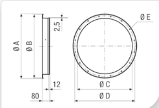
Maße [mm]
