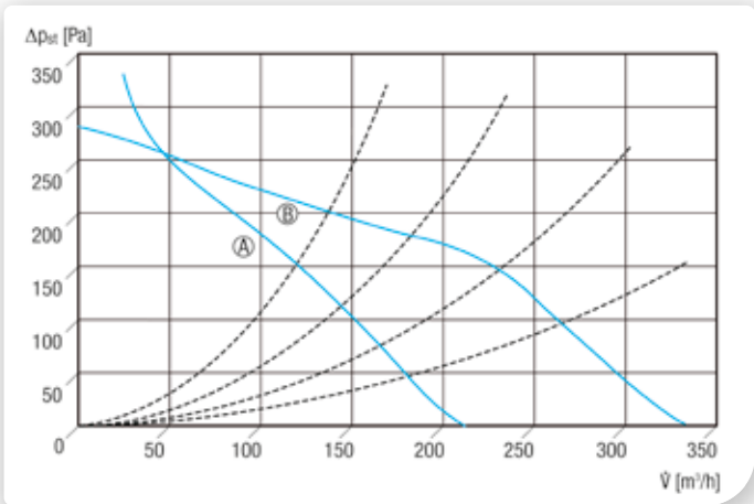
Ⓐ AWW 10 Ⓑ AWW 15
