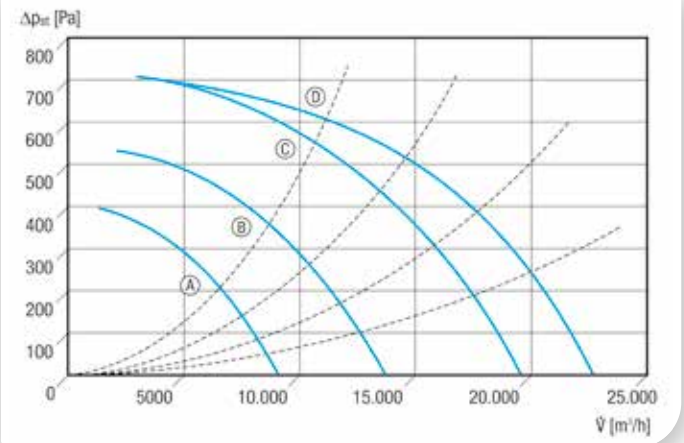
Ⓐ DRD H 56/6 Ⓑ DRD H 63/6 Ⓒ DRD H 75/6 Ⓓ DRD H 80/6
