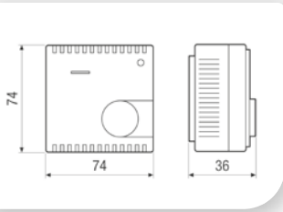
Maße [mm]
