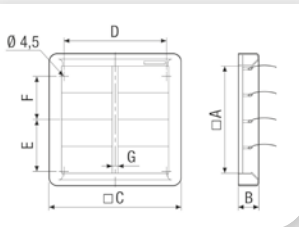
Maße [mm] AS 35 bis AS 60
