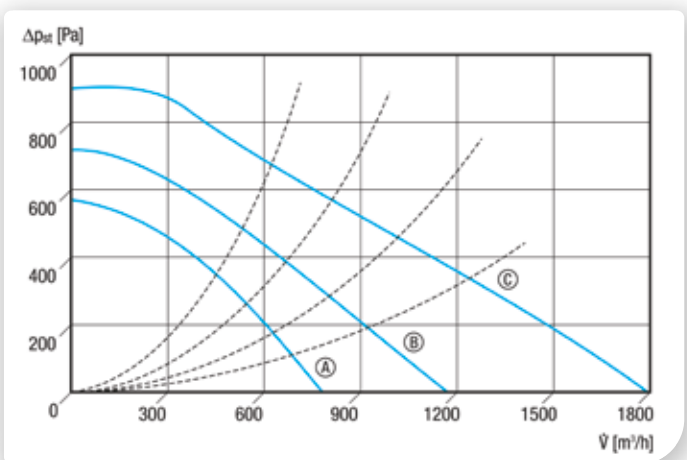
Ⓐ ESR 20-3 EC Ⓑ ESR 25-3 EC Ⓒ ESR 31-3 EC
