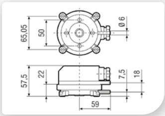
Maße [mm]
