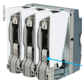
Connection terminal without field deflector
