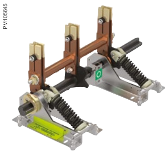
Earthing switch
