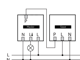
theMura S180-100/theMura S180 Slave
