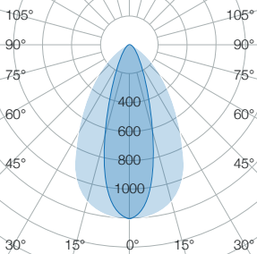
ClickLUX ROCKET SL 25° x 60°
