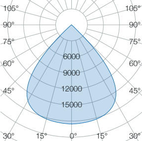
ClickLUX ROCKET SL 90°
