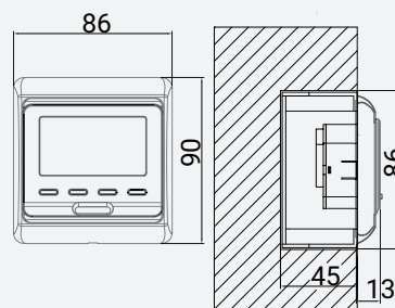
Displayed model TSET103 - Thermostat ST.2 white
