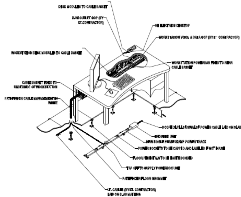
TYPICAL DESK SMALL POWER ARRANGEMENT
