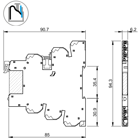
Borne Push-in
