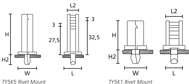
TY5K5 Rivet Mount
