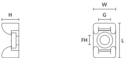
KR6G5, KR8G5 and CTM (side view)
