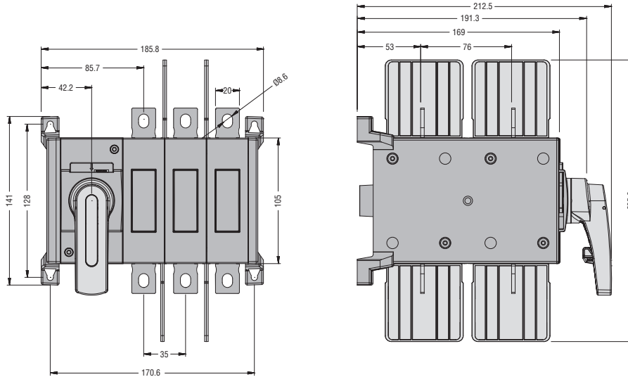
GLC0100T4C1UL - GLC0200T4C1UL
