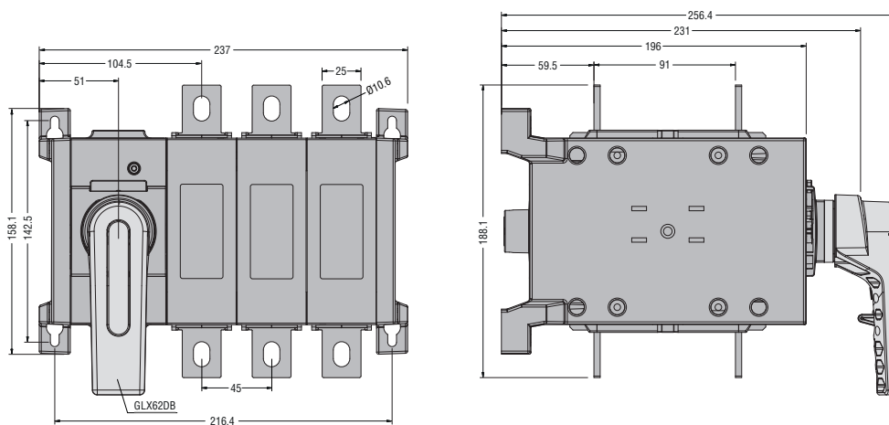
GLC0320C1...GLC0500C1
