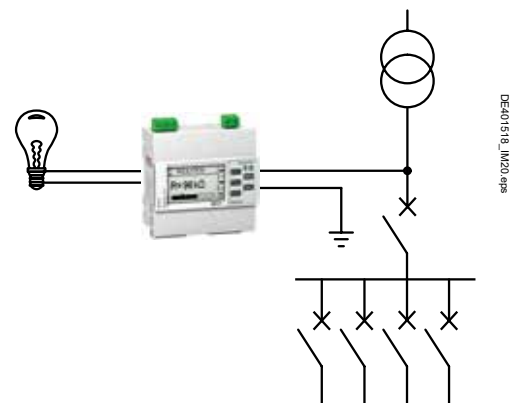
Example of simple insulation monitoring system
