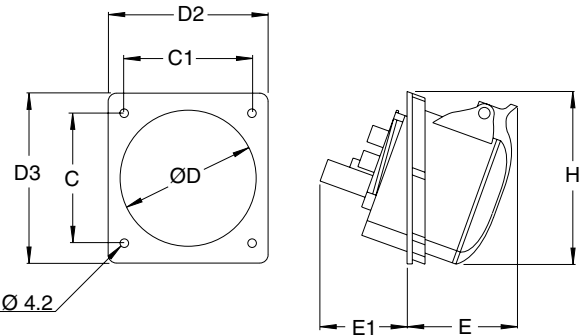
Dimensions (mm)
