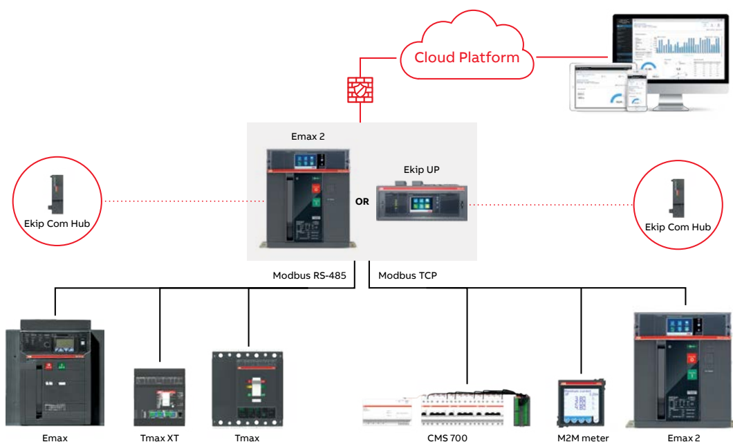
Example of a typical architecture
