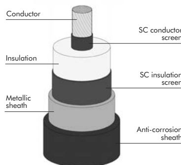
Cable components
