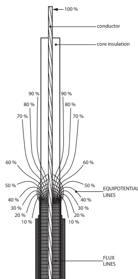
Stress cable
