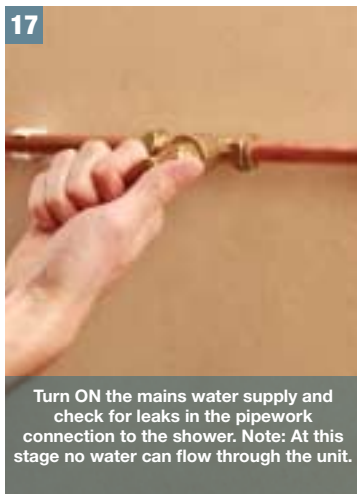
Note: We recommended that a WRAS listed isolating valve be fitted between the rising main and the unit for any future service needs without having to turn off the house water at the stop valve.
