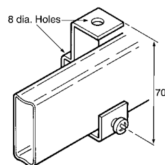
Universal bracket
