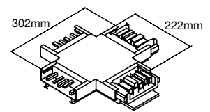
Intersection 125–250A
