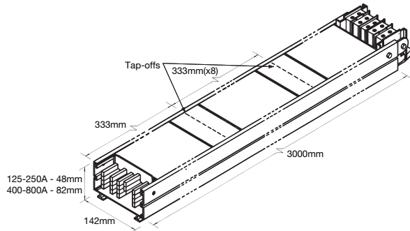
Straight length
