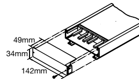
Endcap
