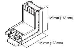
Angle inside edge (125A/250A) Figures in brackets (400A/630A/800A)
