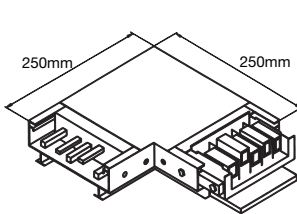
Angle flat left hand
