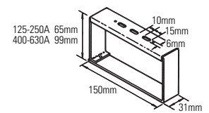
125-630A Universal fixing bracket
