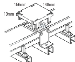
Joint cover
