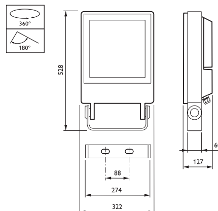
Decoflood 2 BVP636/646
