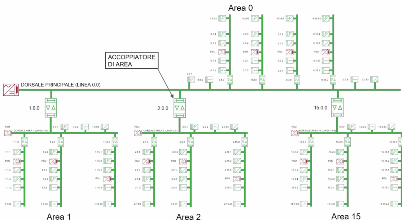
Figura 15. – Network KNX
