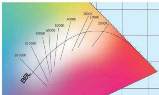
Figura 25. – BBL - Black Body Line
