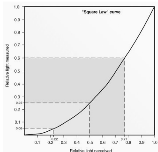
Figura 24. – Curva Square Law
