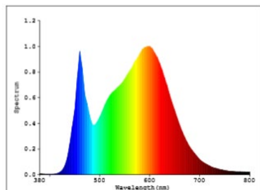
SubstiTUBE (4000K)
