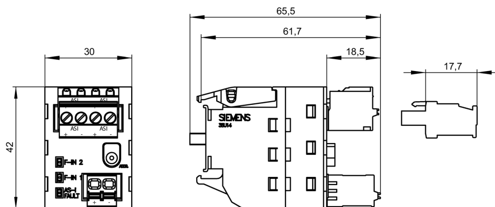
Figura 13-1 3SU1400-1EC10-2AA0_ASI F-Adapter SC+SP 2F-DI+1DO_de
