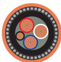
LV power
