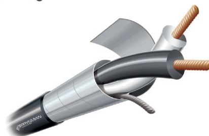
Single pair instrumentation cable.
