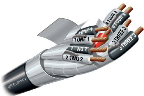
Instrumentation cable with individual and collective screens.
